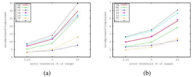
Fig. 2. Compression ratios for a) Humidity and b) Wind Direction datasets.
