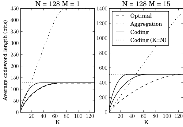
Fig. 1. Comparison of the average codeword length for different protocols. The performance of coding is bounded by the two lines represented in the plot.
