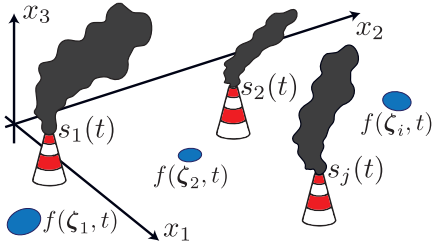
Fig. 2. A sketch of the sensing scenario. The M smokestacks are at known locations \{\xi_j\} . The sensors are represented as blue circles and are located at \{\zeta_i\} . We estimate the flow of substance that is released by each smokestack s_j(t) .
