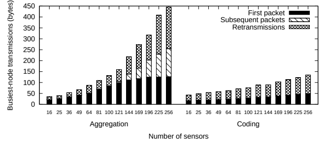
Fig. 2. Number of bytes transmitted by the busiest node including link layer headers. Since aggregated packets sometimes exceed the MTU they need to be fragmented, the part of bytes belonging to additional fragments is indicated as subsequent packets.
