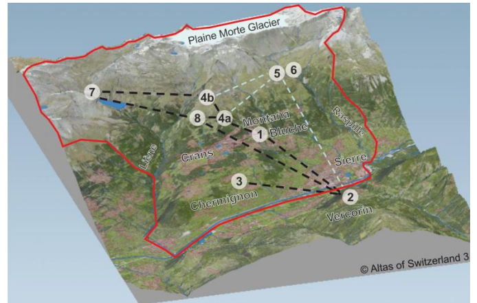
Figure 2. Wireless mesh testbed with nine nodes and interlinks of up to almost 10 km serving the study area of the MontanAqua project in Valais, Switzerland with broadband network access.
