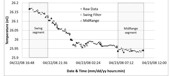
Fig. 1. Different data segments are better approximated by different models.
