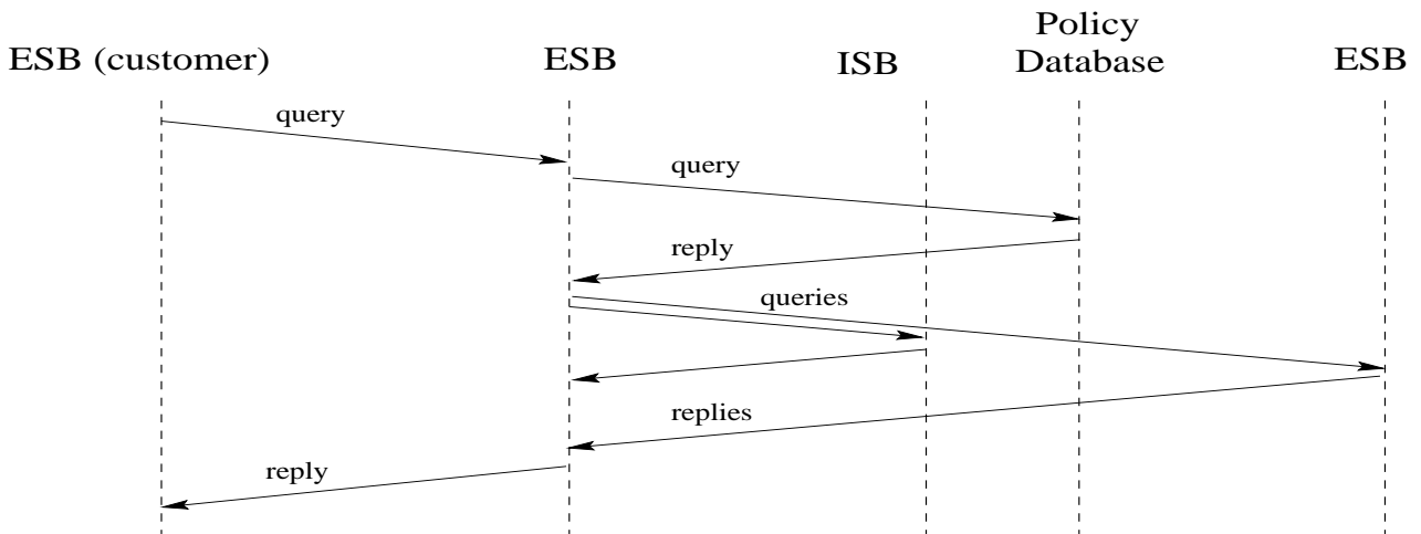
FIGURE 13. The successful ESB-ESB query
