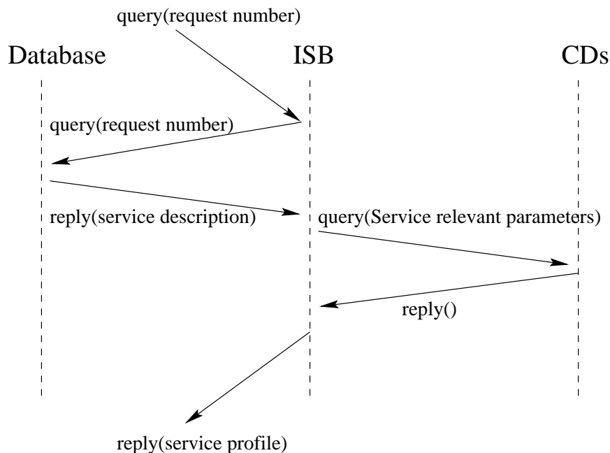
FIGURE 10. A service query
