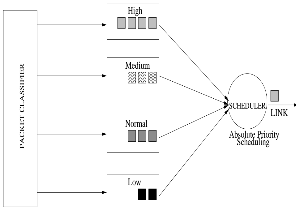
FIGURE 18. Priority Queuing
