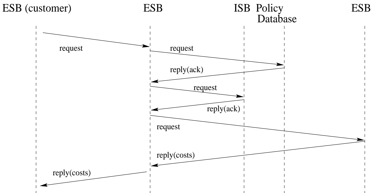
FIGURE 14. A successful ESB-ESB request
